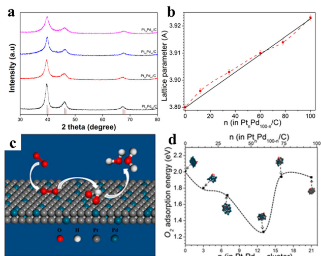
Fig. 27 (a) XRD patterns of Pt 12 Pd 88 /C, Pt 35 Pd 65 /C, Pt 60 Pd 40 /C, and Pt 78 Pd 22 /C nanowires (b) lattice parameters for PtnPd 100-n NWs/C on the relative composition of Pt%, the solid black line is according to Vegard's law based on the lattice parameters of Pt and Pd. (c) Schematic illustration of the catalytic synergy for the ORR over PtPd nanowires featuring the (111) facet. (d) Adsorption energy for molecularly adsorbed O on PtnPd 21-n clusters ( n = 1-21 ) obtained by DFT calculations. Reprinted with permission from ref. 112. Copyright 2020 from the American Chemical Society.
