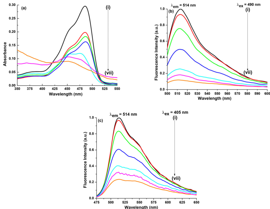
Fig. 1 (a) Absorption spectral profile of NaFlu with GO in water: (i) NaFlu, (ii) NaFlu + 3 mg mL -1 GO, (iii) NaFlu + 15 mg mL -1 GO, (iv) NaFlu + 25 mg mL -1 GO, (v) NaFlu + 35 mg mL -1 GO, (vi) NaF + 60 mg mL -1 GO and (vii) NaFlu + 90 mg mL -1 GO. Fluorescence emission spectra of NaFlu with GO in water (b) \lambda_{\text{ex}} = 490 \text{ nm} and (c) \lambda_{\text{ex}} = 405 \text{ nm} : (i) NaFlu, (ii) NaFlu + 3 mg mL -1 GO, (iii) NaFlu + 15 mg mL -1 GO, (iv) NaFlu + 25 mg mL -1 GO, (v) NaFlu + 35 mg mL -1 GO, (vi) NaFlu + 60 mg mL -1 GO and (vii) NaFlu + 90 mg mL -1 GO.
