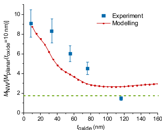
Fig. 4 Experimental and modelled excitation enhancement for \lambda = 640 nm as a function of t_{\text{oxide}} . A M_{\text{planar}} reference for t_{\text{oxide}} = 10 nm is assumed here. For the experiments, we used GaP NWs with d = 109 \pm 10 nm. For the modelling, we assumed a fixed d = 110 nm. Values above the dotted green line correspond to enhancement on the NW compared to a free fluorophore in water.
