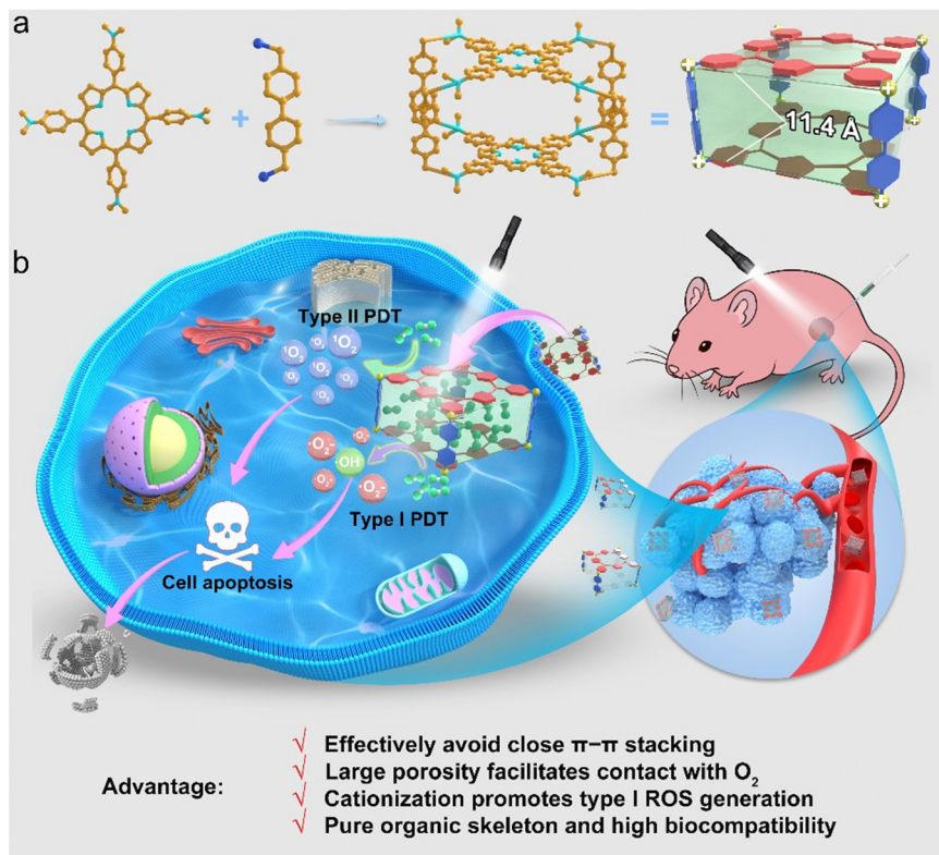
Scheme 1 (a) Schematic of the synthesis of the Py-Cage; (b) schematic of the working mechanism of the Py-Cage: the Py-Cage enhances the generation of type I ( \cdot OH and \cdot O_2 ) and type II ( ^1O_2 ) ROS under white light irradiation to induce cell apoptosis and death for PDT applications.
