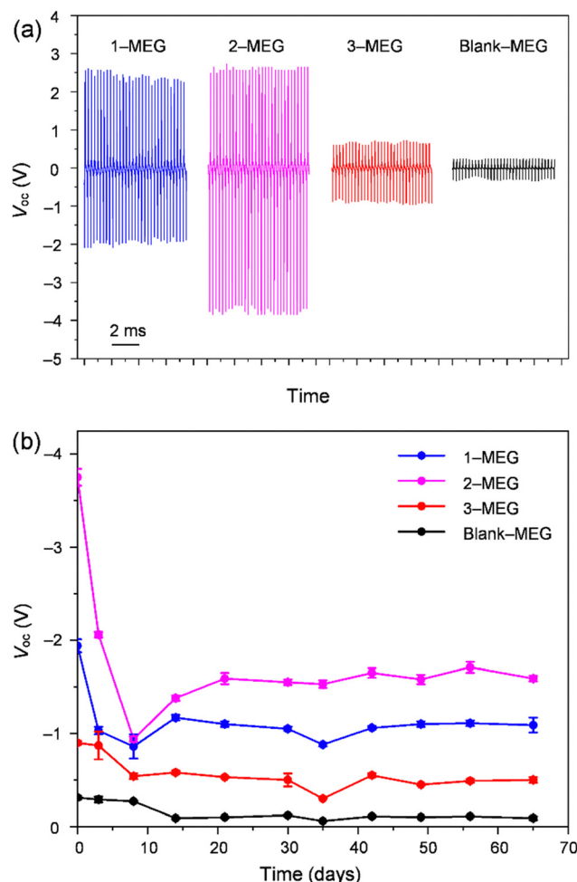
Fig. 4 (a) Open-circuit voltage ( V_{oc} ) characteristics of fabricated mechanoelectric generators (MEGs) with 1 , 2 , 3 , and a blank under continuous vibration at 53 Hz; (b) decay graph of MEG devices showing the stability of the average negative output voltage ( V_{ave-n} ) of the devices under continuous vibration at 53 Hz on the time scale (days).
