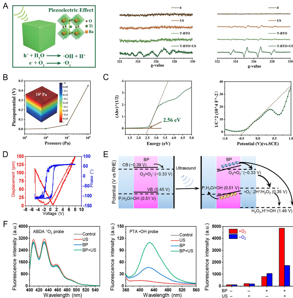
Fig. 12 (A) Schematic and ESR spectra of •O 2 - and •OH generation by tetragonal BaTiO 3 (T-BTO) nanoparticle-mediated piezoelectric effect. (B) Cavitation pressure-dependent piezo-potential of BaTiO 3 nanocrystals and COMSOL simulation for piezopotential distribution. (C) Bandgap and Mott Schottky spectra of T-BTO nanocrystals. 108 Copyright 2019, WILEY-VCH. (D) Height phase hysteresis loop and amplitude butterfly loop for BPs. (E) Changes in the inherent energy band of BP nanosheets after ultrasonic excitation. (F) Assessment of ROS production capacity. 109 Copyright 2020, the American Chemical Society.
