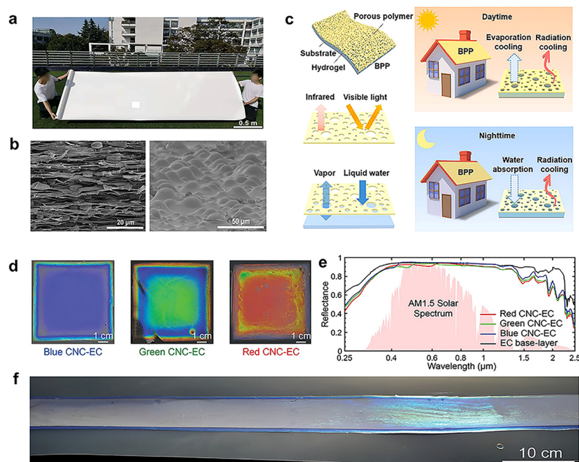
Fig. 6 (a) Photograph of the super-large-scale hierarchically porous film. (b) The SEM image of cross-sectional porous film with hierarchical eye-like air pores inside (left) and the PMMA micro-hemisphere coated on the porous film (right). Reproduced with permission from ref. 78. Copyright 2022, Wiley-VCH GmbH. (c) Optical performance and vapor evaporation of the bilayer porous polymer for intelligent building cooling. Reproduced with permission from ref. 79. Copyright 2021, Elsevier (d) macroscopic images and (e) spectral UV-Vis-IR reflectivity of EC film and blue, green, and red CNC-EC bilayer films. (f) large area film under natural light. Reproduced with permission from ref. 83. Copyright 2022, Wiley-VCH GmbH.
