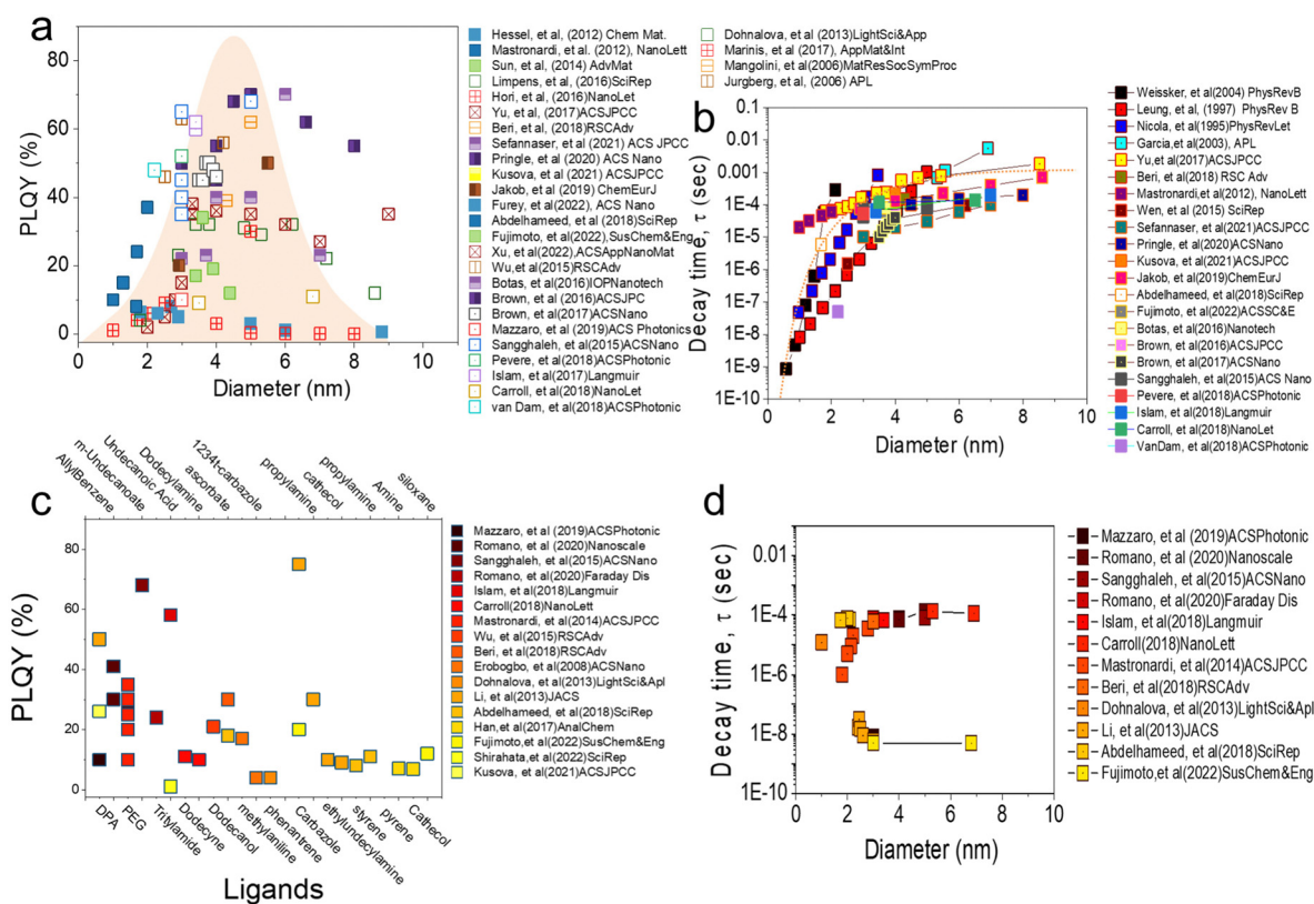
Fig. 2 (a) The relationship between PLQY and diameter for alkyl-functionalized SiQDs reported by various authors in recent years. It can be seen that most papers report PLQY for particles between 1–10 nm with distribution patterns mostly concentrated between 2.5–6 nm. The imaginary distribution curve in the centre of the figure provides insight that most authors are working within this range. (b) The relationship between PL decay and the diameter of SiQDs reported by the authors in graph (a). It can be seen that the PL decay of alkyl-functionalized SiQDs is size dependence ( 10^{-9} to 10^{-6} s). (c) The relationship between PLQY and ligand for non-alkyl functionalized SiQDs reported by various authors in recent years. As in (a), the particle size is in the same range but the PLQY value can be very much different depending on the type of ligand connected to the SiQDs core. Finally (d) is a graph of the relationship between PL decay and diameter as supporting (c). The PL decay reported by these authors is in the nano second range regardless of particle size, however there are also reports that it depends on particle size.
