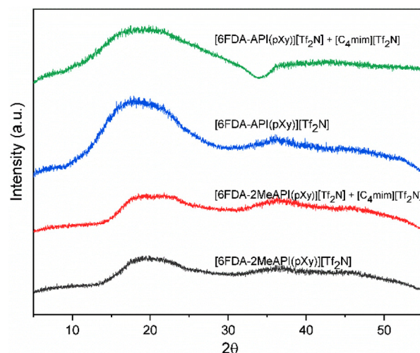
Fig. 14 XRD profiles of 6FDA C(2)–H and C(2)–Me, both neat and composite, Pls.
