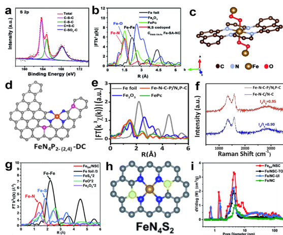
Fig. 9 (a) High-resolution XPS spectra of S 2p. 68 (b) Magnitudes of k^3 -weighted Fourier-transformed EXAFS data of Fe atoms. 68 (c) The structure of the active site in N, S co-doped C PANI-TA-Fe Fe-SA-NC. 68 (d) Schematic diagram of the edge-type FeN 4 P 2 site. 74 (e) FT-EXAFS curves of Fe-N-C-P/N, P-C and reference materials. 74 (f) Raman spectra of Fe-N-C-P/N, P-C and Fe-N-C/N-C. 74 (g) FT-EXAFS spectra of Fe SA /NSC and other references. 75 (h) Model of FeN 4 S 2 . 75 (i) Pore size distribution curves of Fe SA /NSC and other catalysts. 75
