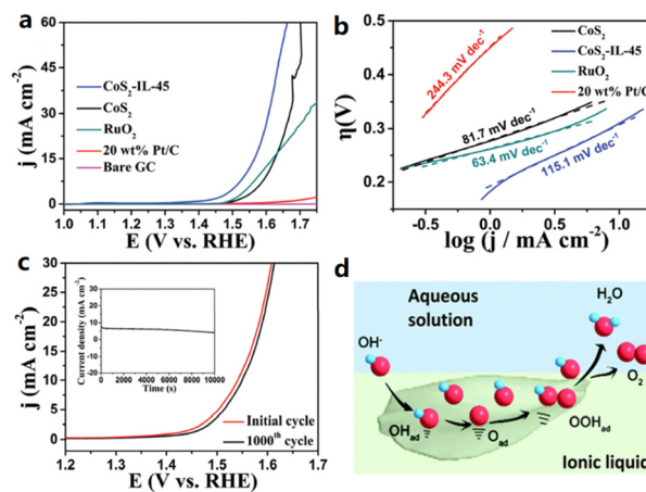
Fig. 3 (a) OER LSV curves of the bare GC electrode, commercial 20 wt% Pt/C, CoS 2 and IL-modified CoS 2 and (b) the derived Tafel plots. (c) OER LSV curves of IL-modified CoS 2 before and after 1000 CV tests. (d) Schematic illustration of the oxidation of water. Reproduced with permission. 46 Copyright 2018, the Royal Society of Chemistry.
