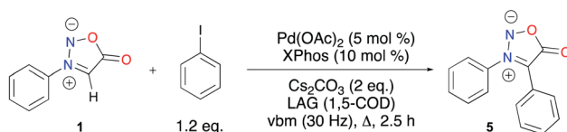
Scheme 2 Mechanochemical palladium-catalyzed C–H activation.
