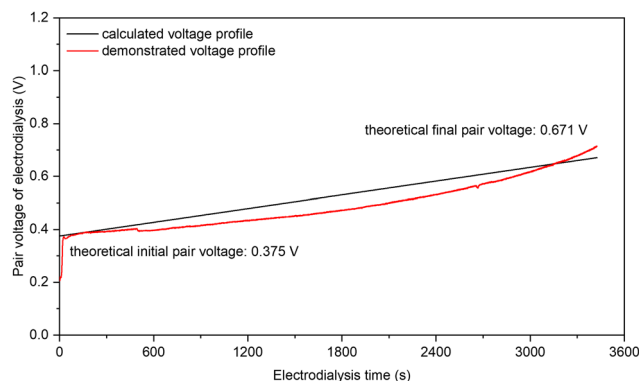
Fig. 4 The voltage profiles of one electro dialysis pair along with electro dialysis time for \text{NO}_3^- concentration. A single electro dialysis pair is constructed by the configuration of “CEM | diluate | AEM | concentrate” in which the CEM and the AEM are FKA-PK-130 and FAA-PK-130, respectively, both from Fuma-Tech; and the diluate and the concentrate are 7.14 mM \text{KNO}_3 (100 ppm \text{NO}_3^- -N) and 2 M \text{KNO}_3 (28 000 ppm \text{NO}_3^- -N), respectively. The key experimental conditions include: 5 \text{cm}^2 as the effective pair area, 1 \text{mA cm}^{-2} as the electro dialysis current density, 10 \text{cm s}^{-1} as the nominal fluid velocity for all channels (60 \text{mL min}^{-1} ), 0.5 mm as the distance between CEM and AEM in the electro dialysis pair, and 75% as the designed \text{NO}_3^- removal (3444 seconds). Note that the applied current density for ED is subject to the threshold set by the “limiting current density” calculated by the Rosenberg and Tirrell equation, 41 and the obtained limiting current density is 4.62 and 1.19 \text{mA cm}^{-2} at the initial (7.14 mM) and the final diluate concentration (1.79 mM), respectively, under our experimental conditions.
