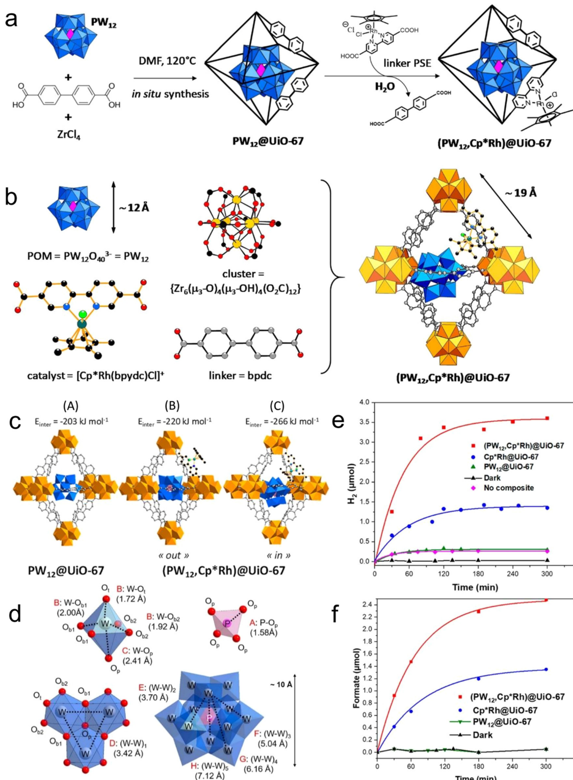
Fig. 11 (a) Schematic of in situ synthesis. (b) Components of (\text{PW}_{12}, \text{Cp}^*\text{Rh})@\text{UiO}-67 . (c) Models of \text{PW}_{12}@\text{UiO}-67 and (\text{PW}_{12}, \text{Cp}^*\text{Rh})@\text{UiO}-67 . (d) Distances between the components of POM. Production rate of (e) \text{H}_2 and (f) \text{HCOO}^- . Reproduced with permission from ref. 166 Copyright 2020, ACS.
