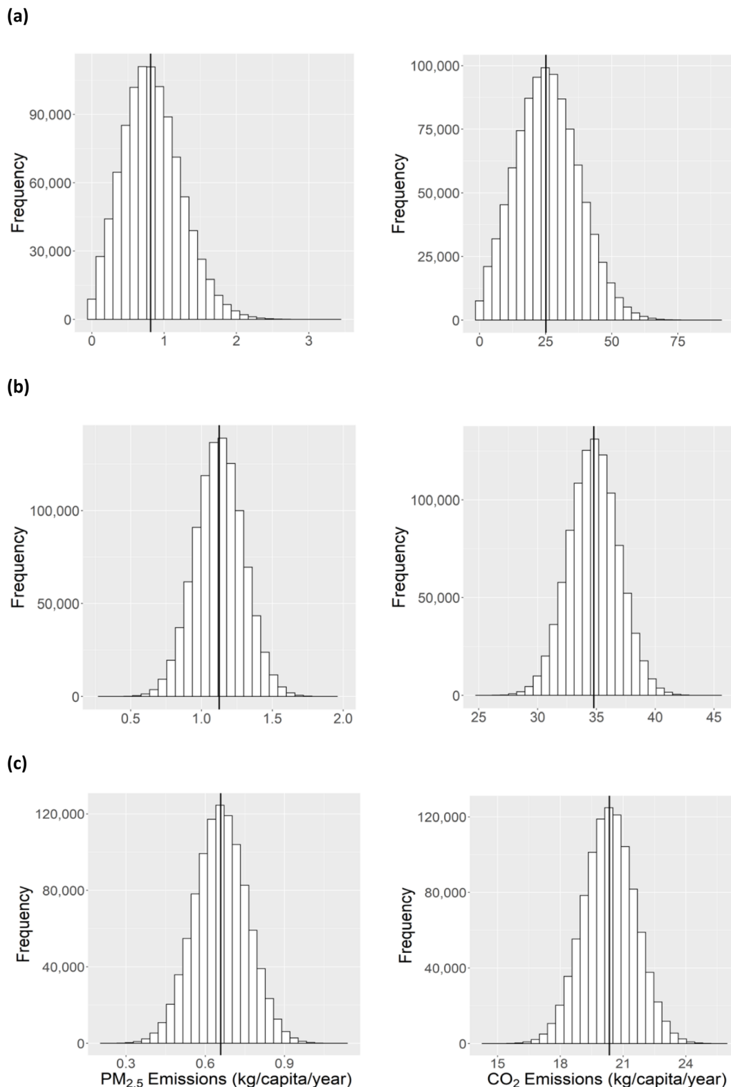
Fig. 2 Particulate matter ( \text{PM}_{2.5} , left) and carbon dioxide ( \text{CO}_2 , right) annual emission estimate distribution from Monte Carlo samplings for (a) the Jalapán region of Jalapa, (b) the city of Jutiapa, and (c) Guatemala city.
