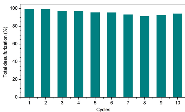
Fig. 6 Reusability of the homogeneous \text{PMo}_4 (7.5 \mu\text{mol} ) catalyst using 0.75 mL of [Bmim]PF 6 extraction solvent, 0.78 mmol of \text{H}_2\text{O}_2 , and 7.5 \mu\text{mol} of \text{PMo}_4 at 70 °C. The results were obtained at 2 h.
