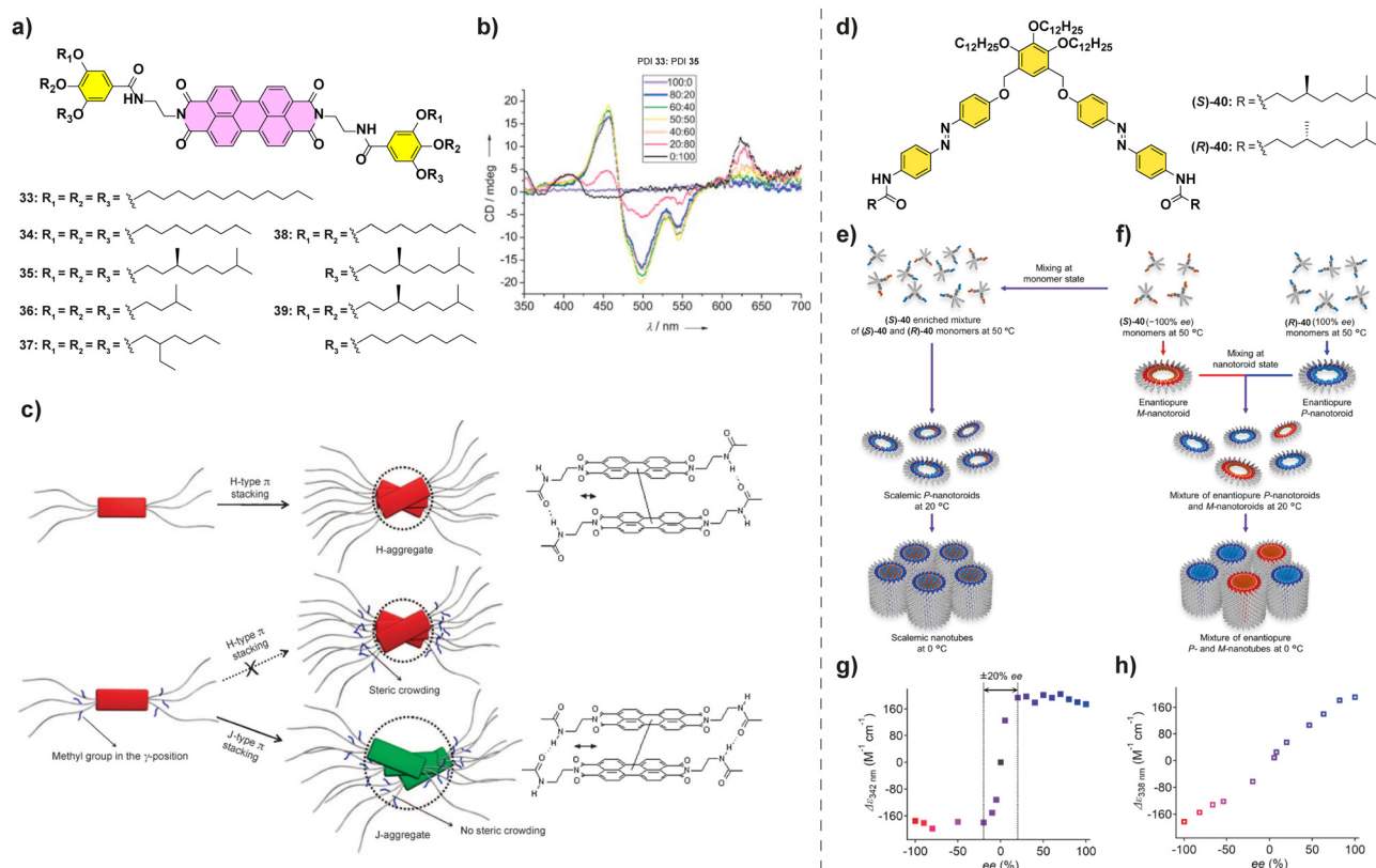
Fig. 20 (a) Chemical structure of PDIs 33–39 . (b) CD spectra of mixtures of PDIs 33 and 35 at different ratios (c T = 10 μM in MCH/CHCl 3 80/20). (c) Schematic representation of the polymerization of PBIs 33–39 into H- or J-aggregates (reproduced from ref. 92 with permission from Wiley-VCH, copyright 2008). (d) Chemical structure of (S)- and (R)-40 . (e) and (f) Schematic representations of the distinct hierarchical organization of (S)-40 and (R)-40 . (g) MR experiment performed in salemic nanotoroids as prepared in (e). (h) MR experiment performed in mixtures of enantiopure nanotoroids as prepared in (f) (c T = 300 μM in MCH) (reproduced from ref. 96 with permission from the American Chemical Society, copyright 2023).
