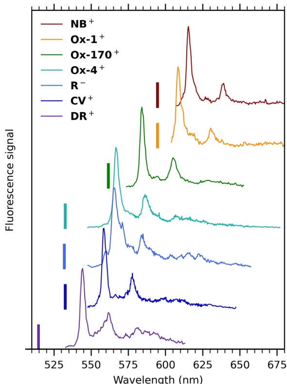
Fig. 6 Dispersed-fluorescence spectra of seven oxazine ions isolated in vacuo measured at cryogenic temperature (100 K). Excitation wavelengths are indicated by vertical bars, and they were 514 (DR + ), 531.3 nm (R - ), 532 nm (CV + , Ox-4 + ), 561 nm (Ox-170 + ) and 594 nm (Ox-1 + , NB + ). The spectrum of DR + is obtained with a lower excitation wavelength than the spectrum in Fig. 4(b) to avoid cutting off part of the main band by the notch filter.
