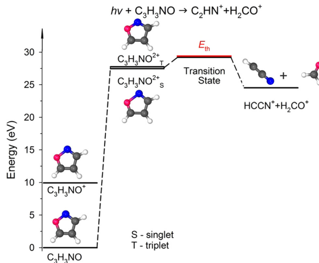
Fig. 6 The simplified potential energy profile for the dissociation of the isoxazole dication into \text{H}_2\text{CO}^+ + \text{HCCN}^+ . The scheme is based on the data presented in Table S1, ESI†.
