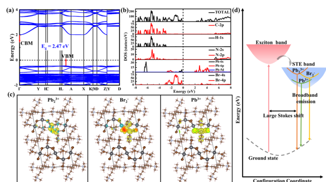
Fig. 4 (a) Calculated electronic band structures and (b) DOS of (HM)Pb 2 Br 6 . (c) Calculated charge density for (HM)Pb 2 Br 6 (Pb 2 3+ STEs, Br 2 - and Pb 3 + STEs) upon crystal lattice perturbation via the Pb–Pb, Br–Br and Pb–Br distances shortening. (d) Configuration coordinate diagram illustrating the luminescence mechanism.
