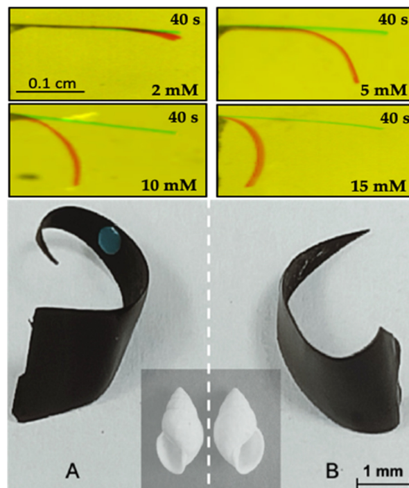
Fig. 6 Top: concentration dependent deflection of Ppy for the enantioselective recognition of L -DOPA on oligo-( S )-BT 2 T 4 hybrid actuator (Copyright © 2020, American Chemical Society). Bottom: picture of the two ( R )- and ( S )-enantiomorphs recovered at the end of the bipolar experiments illustrating the transmission of molecular chirality to the macroscopic scale (Copyright © 2020, American Chemical Society).
