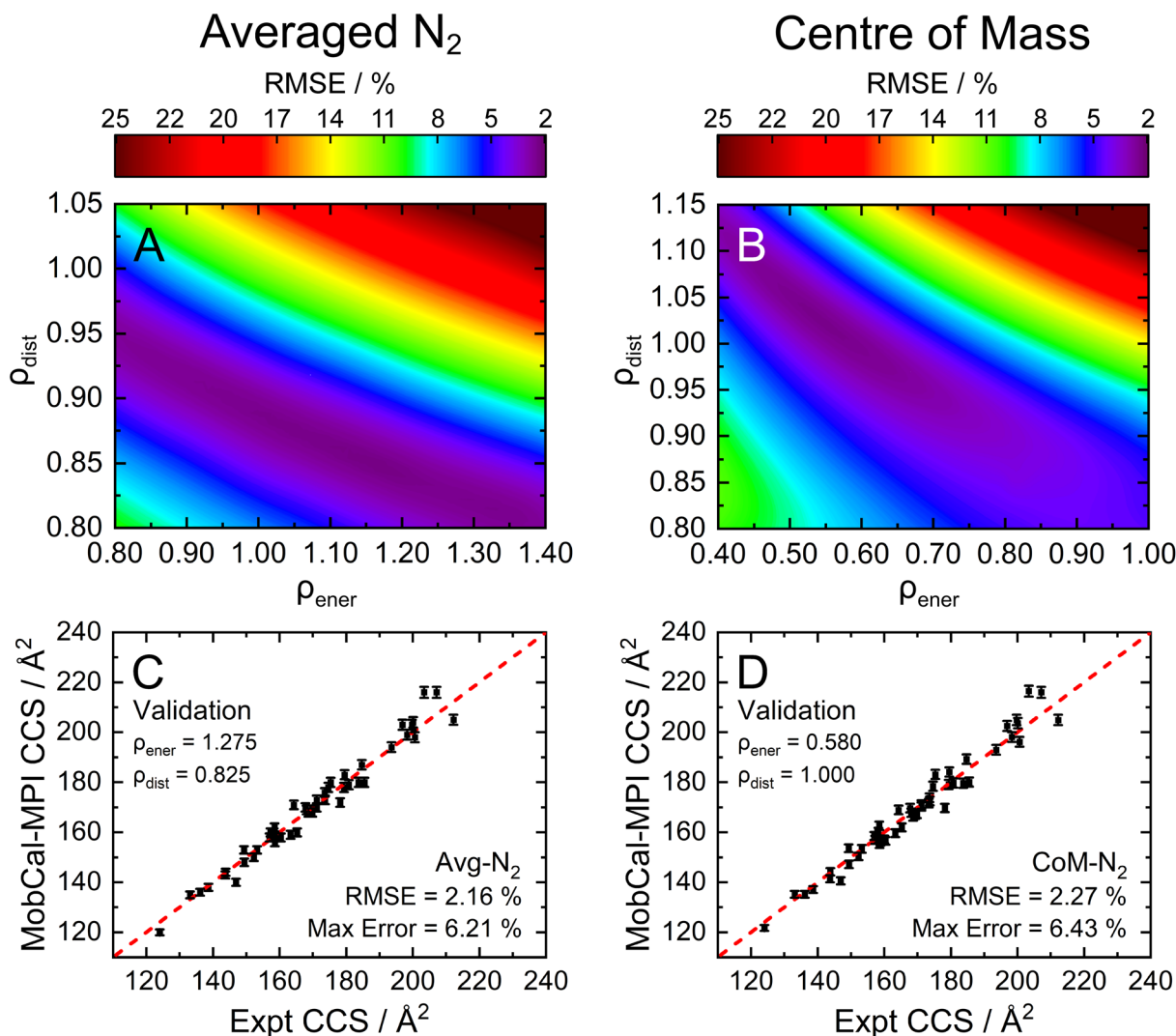
Fig. 3 The RMSE, shown as a contour plot, for the optimization of \rho_{\text{dist}} and \rho_{\text{ener}} using the (A) Avg- N_2 or (B) CoM approach for the calibration set (162 molecules). To validate the accuracy of (C) Avg- N_2 or (D) CoM approaches, we employed the values of \rho_{\text{dist}} and \rho_{\text{ener}} yielding the lowest RMSE to calculate the CCS of 50 distinct molecules that were not present in the calibration set (validation set). All CCS calculations were performed at 298 K with itn = 5 , inp = 104 , and imp = 512 .
