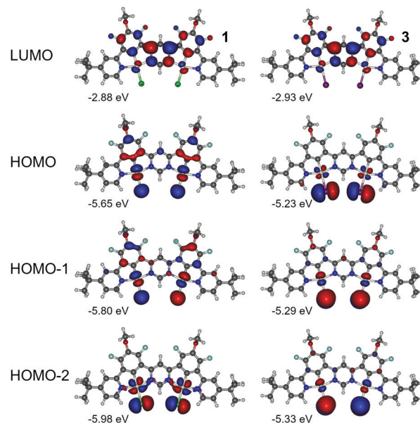
Fig. 8 Molecular orbital contour plots at the B3LYP/dev2-TZVP/ZORA level for diplutonium complexes 1 and 3 .
