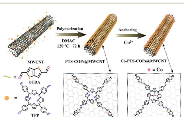
Fig. 1 Schematic illustration of the pyrolysis-free synthesis of the Co-PTS-COPs@MWCNT hybrid.
