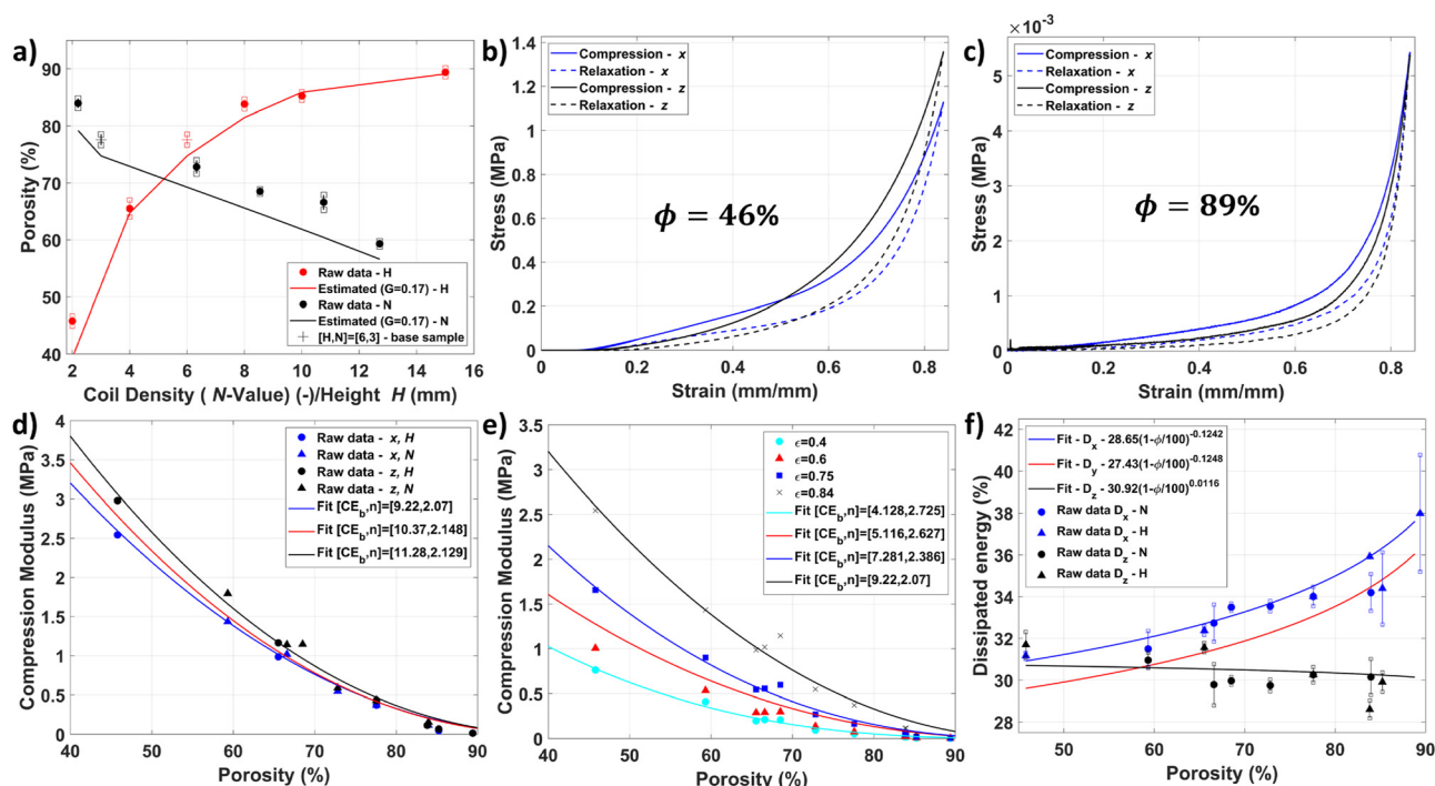
Fig. 4 (a) Porosity versus height ( H ) and coil density ( N -value) with the base sample at [H, N] = [6.3] , (b and c) stress-strain curve at 46% and 89% porosity, (d and e) segment modulus of compression versus porosity for different axes at maximum strain (d) and different levels of strain (e), and (f) the energy dissipation versus porosity.
