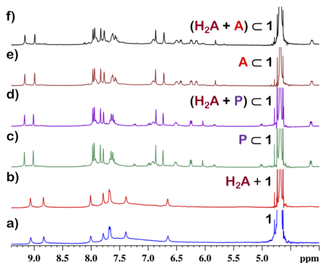
Fig. 6 Partial ^1\text{H} NMR stack plot of (a) 1 , (b) \text{H}_2\text{A} + \text{1} ( \text{H}_2\text{A} = 9,10-dihydroanthracene), (c) \text{P} < \text{1} (P: phenanthrene), (d) (\text{H}_2\text{A} + \text{P}) < \text{1} , (e) \text{A} < \text{1} (A: anthracene) and (f) (\text{H}_2\text{A} + \text{A}) < \text{1} in \text{D}_2\text{O} showing the selective encapsulation of A and P.
