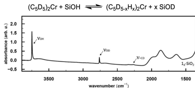
Fig. 3 Top: Proposed reaction for the interaction of 1 d10 with surface OH groups, resulting in D exchange of deuterated Cp rings. Bottom: IR spectrum of D-labeled 1-SiO 2 -1 . In addition to the =CD band, consistent with the deuterated Cp ring, the Si-OD band arises from the H/D exchange with the silica surface.
