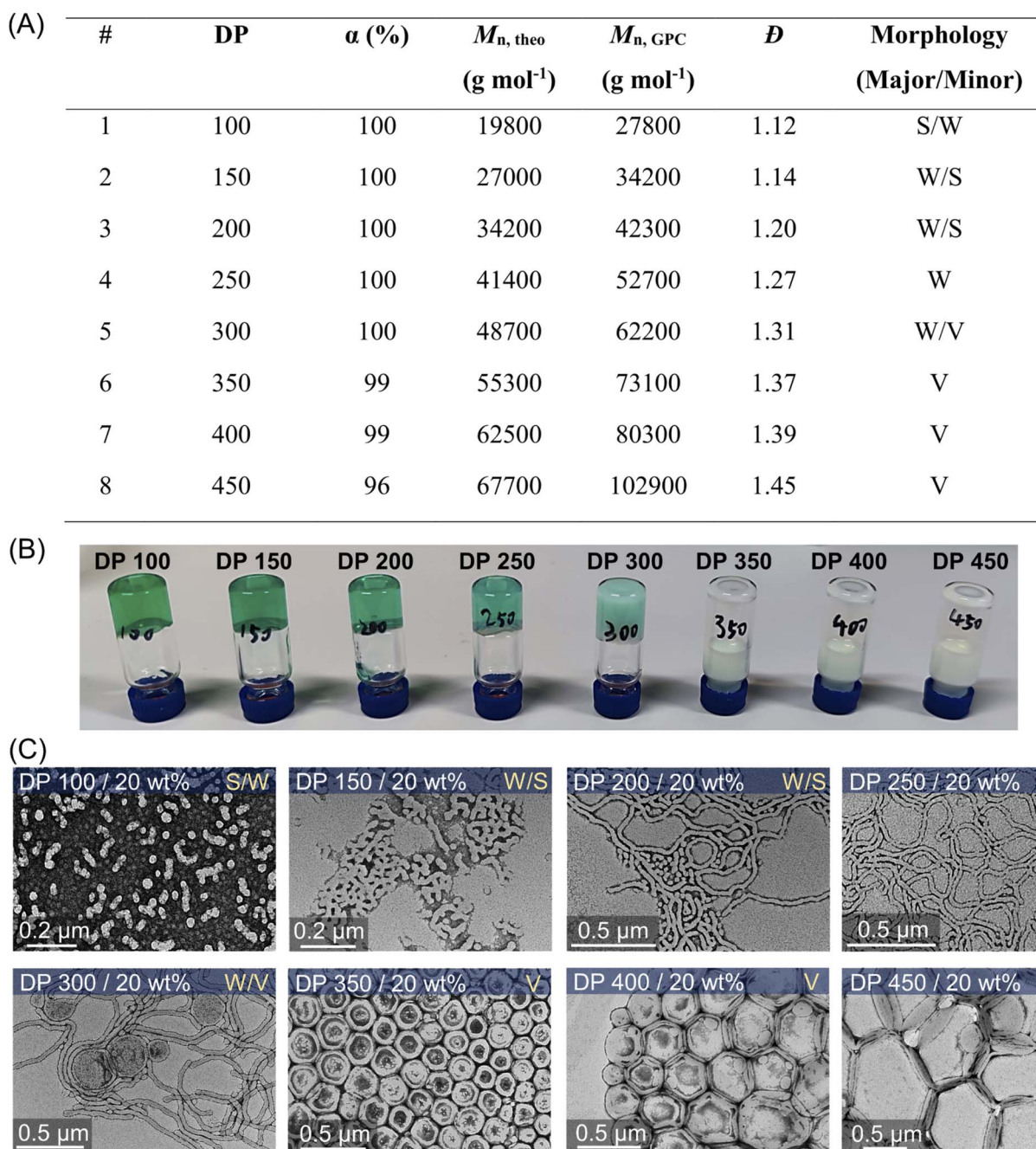
Fig. 5 (A) ZnPcS 4 - mediated dispersion photopolymerization of HPMA by varying target DPs from 100 to 450 at 20 wt% total solids content. Polymerizations were conducted under the irradiation of NIR light ( \lambda_{\text{max}} = 730 nm; 60 \text{ mW cm}^{-2} ) for 24 hours without prior deoxygenation in water at a fixed reaction stoichiometry of [PEG 113 -CDTPA] : [TEOA] : [ZnPcS 4 - ] = 1 : 4 : 0.02. (B) Digital photos of photo-RAFT dispersion polymerization of HPMA with varying target DPs from the same reaction in (A). (C) Corresponding TEM images showing the major and minor morphologies of self-assembled polymeric nanoparticles (S: sphere, W: worms, and V: vesicles).
