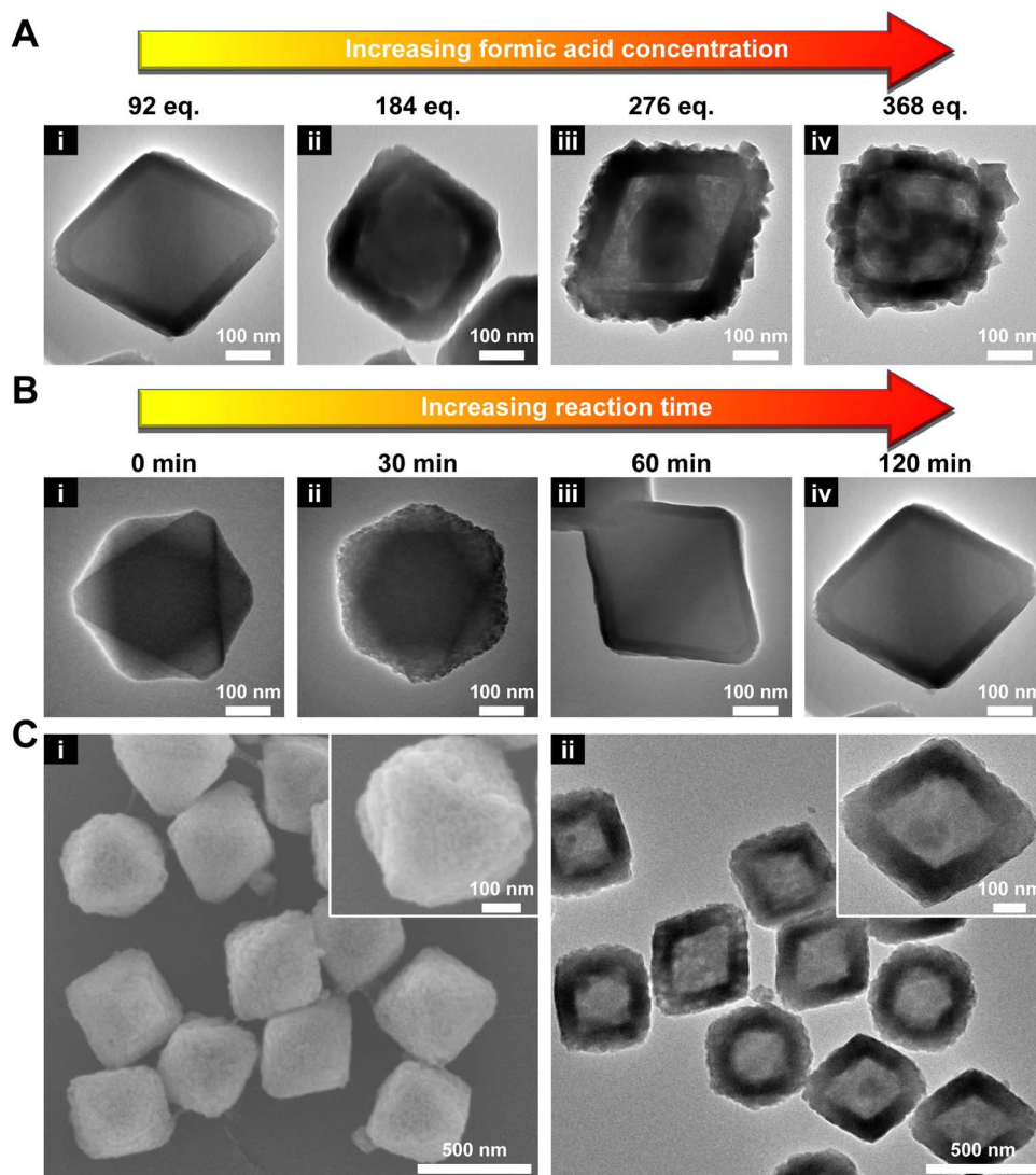
Fig. 1 (A) TEM images of UiO-66@MOF-801 synthesized with various amounts of formic acid. (B) TEM images of UiO-66@MOF-801 obtained after various reaction times. (C) SEM (i) and TEM (ii) images of MOF-801(h).
