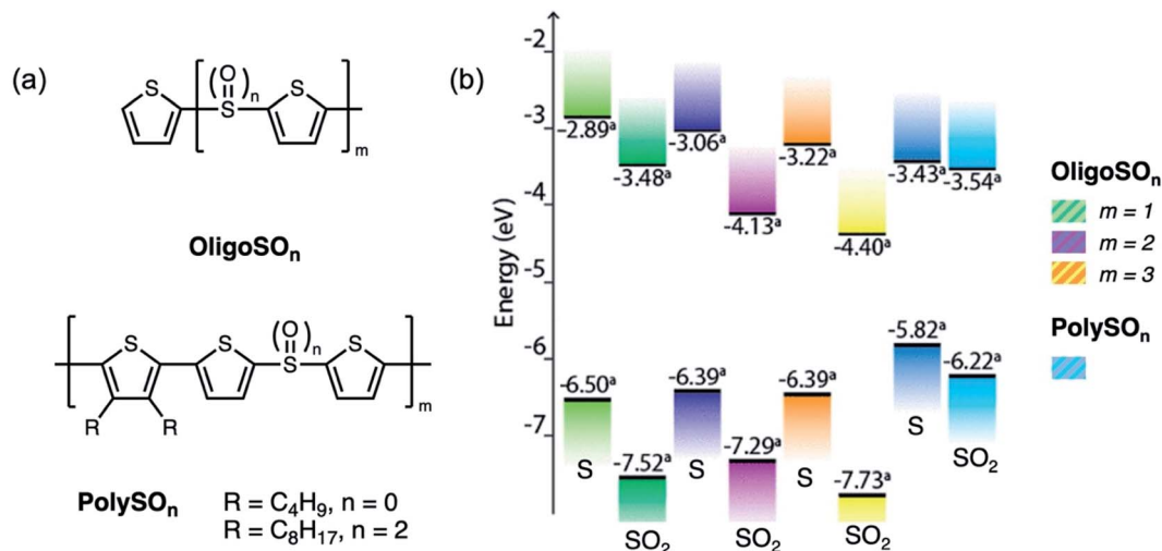
Fig. 10 (a) Structures of thiophene-based oligomers OligoSO n and polymers PolySO n containing a sulfur bridge ( n = 0, 2) reported by our group. (b) Calculated frontier energy levels obtained from cyclic voltammetry measurements and UV-vis absorption spectra. Adapted with permission from ref. 49. Copyright 2017 American Chemical Society.
