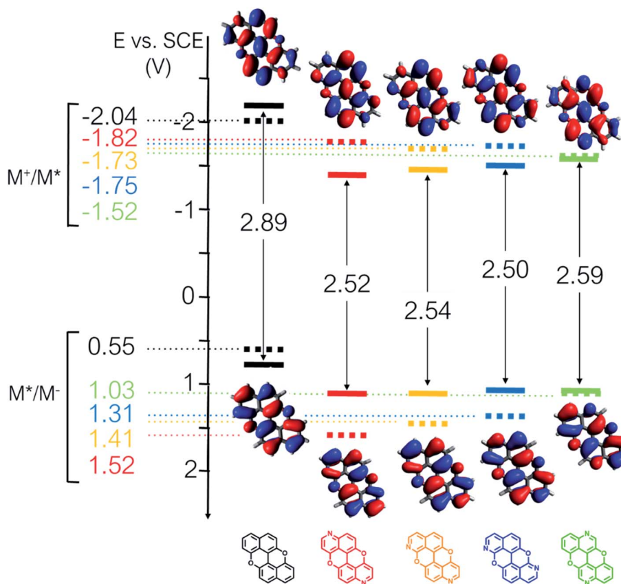
Fig. 6 Redox potentials vs. SCE of PXX, 3,9- N,N -PXX, 1,9- N,N -PXX, 1,7- N,N -PXX and 4,10- N,N -PXX estimated from the CV data obtained in ODCB. Dashed lines: reduction ( E_{M^*/M^-} ) and oxidation ( E_{M^+/M^*} ) potentials of the singlet excited states estimated using the optical band gap measured in toluene. 6 Inserts: DFT calculated HOMO (bottom) and LUMO (top) lobes. 6
