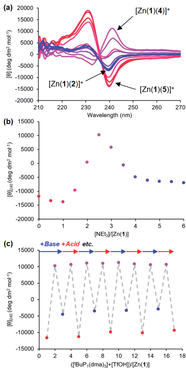
Fig. 9 (a) CD spectra of Zn(1)·2ClO 4 (c 0 = 0.25 mM) with 2-H (1 eq.), 4-H (1 eq.) and 5-H (1 eq.) in MeCN with addition of NEt 3 (0.0 → 6.0 eq.) in 0.5 eq. increments; (b) molar ellipticity at 240 nm with addition of NEt 3 ; (c) molar ellipticity at 240 nm with alternating addition of t BuP 1 (dma) 3 (→) and TfOH (→) in 1 eq. increments.
