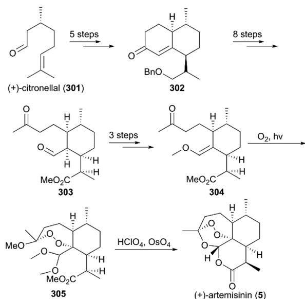
Scheme 29 Total synthesis of (+)-artemisinin by Zhou.
