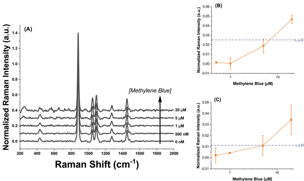
Fig. 8 SERS Intensity profile for APTES functionalized (AuNR@Full) particles (A) for concentrations between 0–20 \mu\text{M} . The values were all normalized to the main ethanol Raman peak for comparison. The asterisks are above the peaks which were analyzed. (B) is the intensity profile for the peak at 240 \text{cm}^{-1} and (C) is the same for the peak at 655 \text{cm}^{-1} . In (B and C), the dashed blue line represents the limit of detection based on the signal with no analyte plus three standard deviations of the average.
