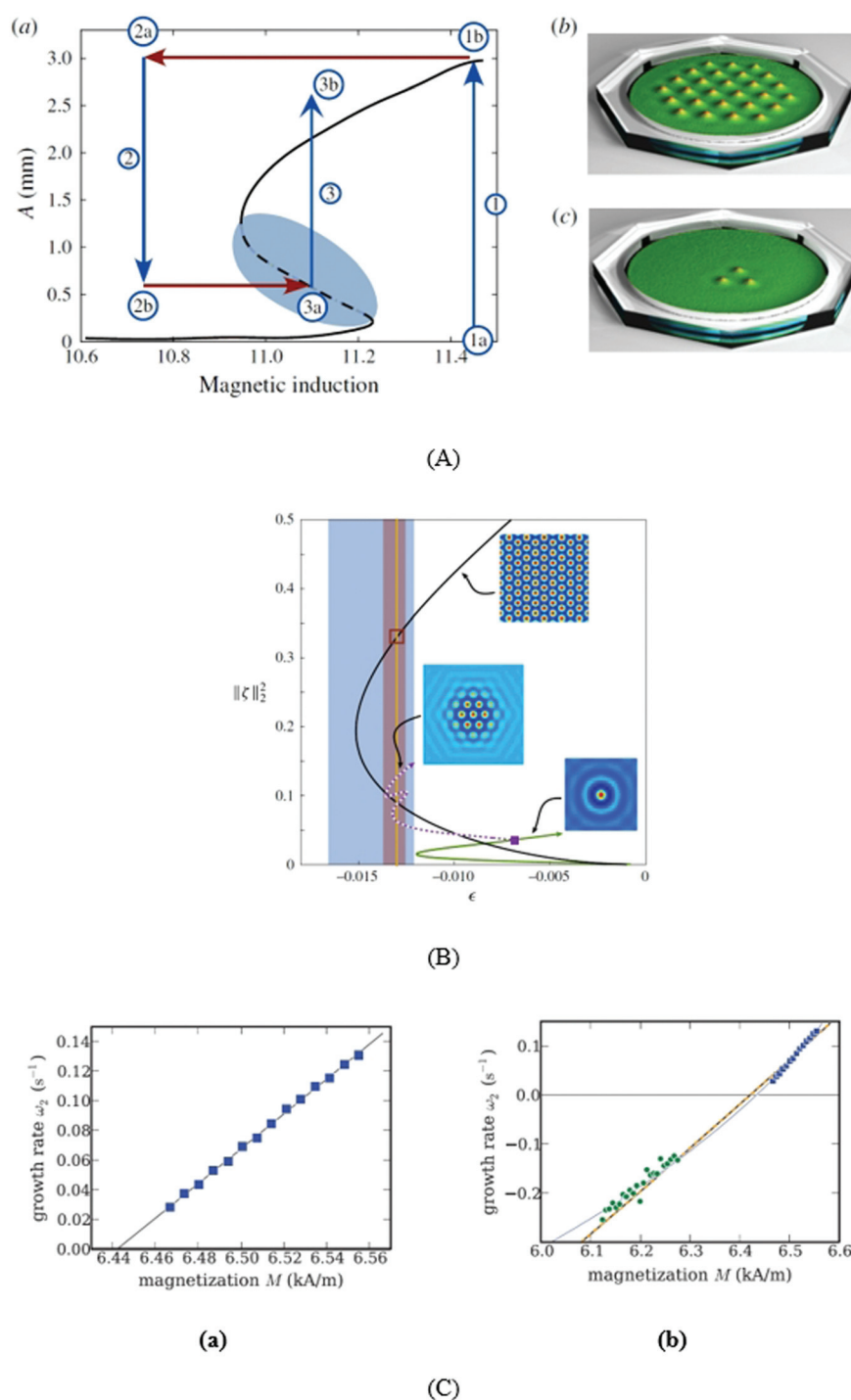
Fig. 31 Rosenzweig instability patterns in a highly viscous ferrofluid. (A) (a) The bifurcation diagram (black line) of this pattern is obtained by a fitting procedure of amplitude equations described in ref. 555 to about 170 000 measured data. Via the path indicated by the arrows, one obtains localized patches, as shown in (c). The magnetic induction B is kept fixed during (1) for a time delay of \tau_1 , and then B is switched to (2) for a time delay of \tau_2 before finally being switched to (3) until equilibrium is reached at point (3b). (b) A reconstruction of the height field of the domain-covering hexagons at point (1b). (c) Gives a reconstruction of the height field of a three-spike patch at point (3b) in the bifurcation diagram. (B) Emergence of a fully localized hexagon patch (dashed purple) bifurcating from a single spike (green) with \mu_r = 2 . There are also plotted the snaking regions of the \langle 10 \rangle (blue) and \langle 11 \rangle planar fronts (red); here, \epsilon denotes the bifurcation parameter, which depends on the relative permeability of the ferrofluid, \mu_r (reproduced from ref. 556 with permission from Cambridge Univ. Press, copyright 2015). (C) Grow and decay of the Rosenzweig pattern in the case of a highly viscous ferrofluid. (a) The linear growth rates \omega_2 (■) from the experiment and the maximal growth rate \omega_{2,m} (solid black line) from theory as a function of the magnetization M . (b) The growth (■) and decay (●) rates \omega_2 of the pattern amplitude as a function of the magnetization M . The symbols represent the measured data. The black dashed line shows a fit of expression of scaling law for \omega_2 to the experimental growth and decay rates (reproduced from ref. 554 with permission from Am. Phys. Soc., copyright 2016).
