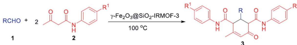
Fig. 30 Synthesis of cyclohexenone derivatives using \gamma\text{-Fe}_2\text{O}_3/\text{SiO}_2/\text{IRMOF-3} catalyst. This figure was adapted with permission from Journal of Catalysis , 2020, 387, 39–46. 188
