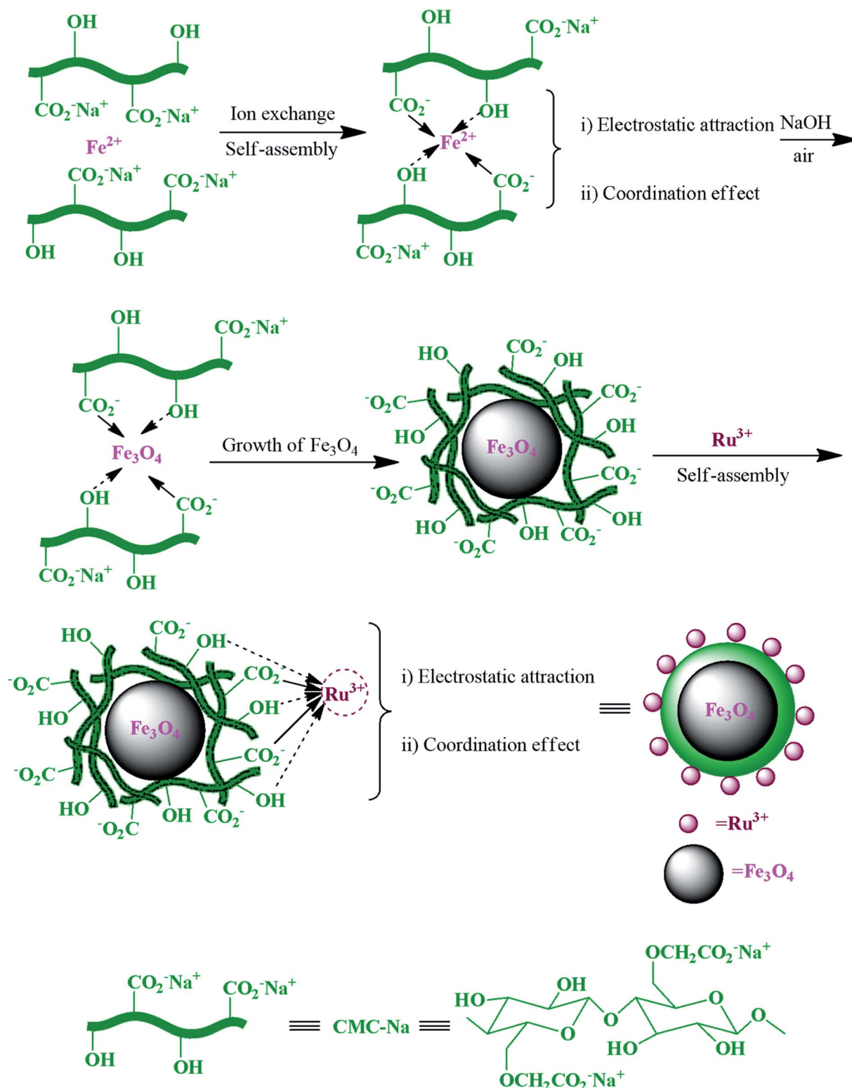
Fig. 16 Schematic of the preparation of magnetic \text{Ru}^{\text{III}}@CMC/\text{Fe}_3\text{O}_4 organic/inorganic hybrid catalyst via self-assembly. This figure was adapted with permission from: Molecular Diversity , 2019, 23, 421–442. 103
