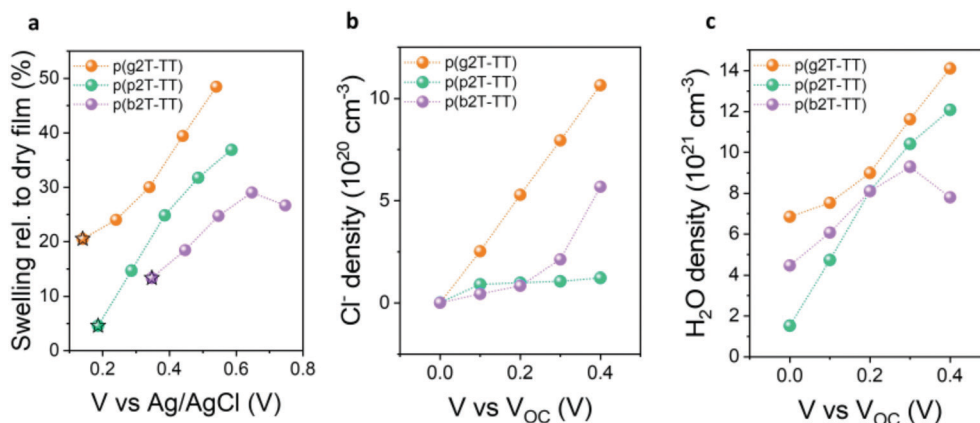
Fig. 3 (a) Polymer swelling relative to the corresponding dry state. Star symbols correspond to the swelling values of the film at V_{OC} conditions ( i.e. , passive swelling). The voltage values are plotted vs. Ag/AgCl. (b) Chloride ion and (c) water molecule density in the conjugated polymer film following electrochemical doping at various potentials against V_{OC} . V_{OC} values are 0.14 V for p(g2T-TT), 0.19 V for p(p2T-TT), and 0.35 V for p(b2T-TT).
