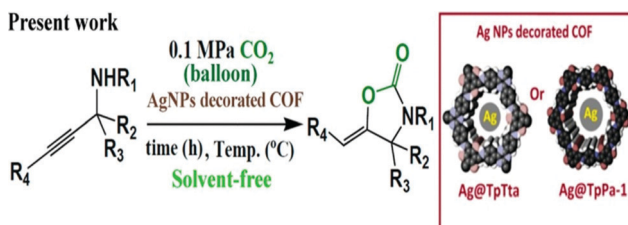
Scheme 37 The synthesis of 2-oxazolidinones using a AgNP-decorated COF. Reproduced with permission from ref. 56; copyright: 2020, ACS Sustainable Chemistry & Engineering.
