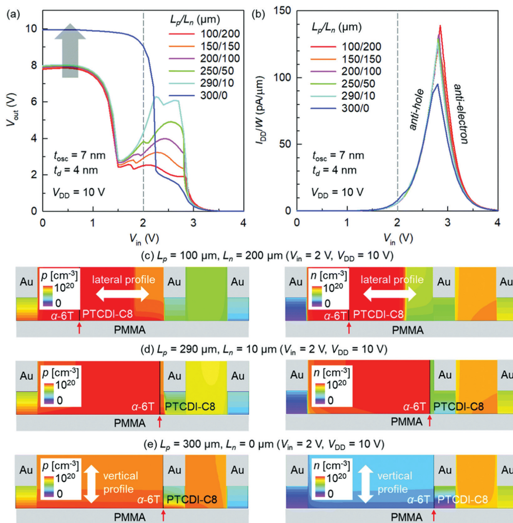
Fig. 11 (a) Voltage transfer curves and (b) I_{D} - V_{IN} curves calculated by theoretical simulation, showing clear L_p/L_n dependence. (c)–(e) Spatial distribution of holes (electrons) on the left (right), depending on L_p/L_n . Reprinted with permission from ref. 34 Copyright 2021 The Royal Society of Chemistry.
