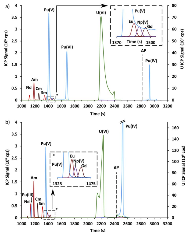
Fig. 4 (a) Electropherogram obtained by CE-Q-ICP-MS for a spent MOX fuel sample with a 120 mmol L -1 \alpha -HMBA electrolyte one day after the end of the oxidation step. (b) Electropherogram obtained by CE-Q-ICP-MS for a spent MOX fuel sample with a 120 mmol L -1 \alpha -HMBA electrolyte seven days after the end of the oxidation step. For both electropherograms, it was necessary to apply 1 bar of pressure in order for Pu(IV) to migrate. The time at which the pressure ( \Delta P ) was applied is symbolized as a dashed line.
