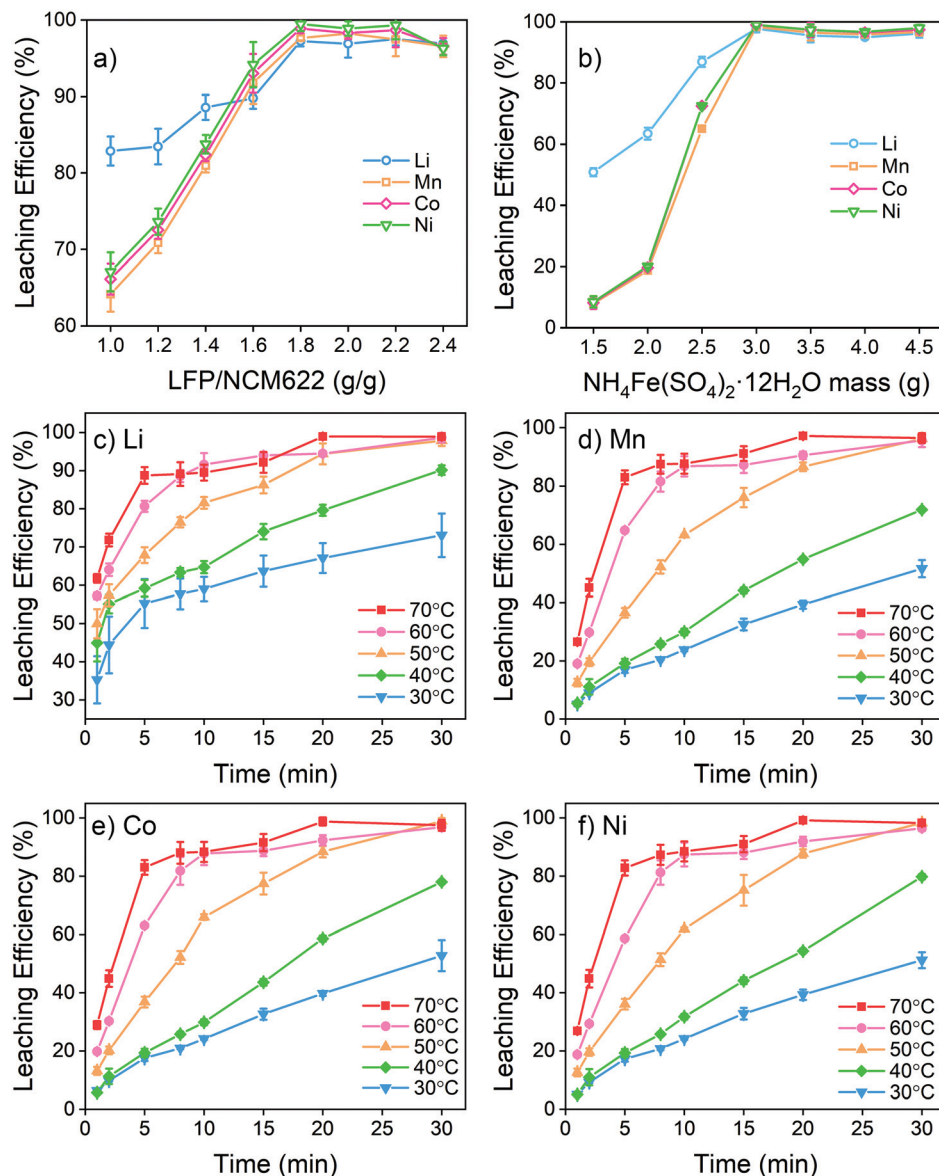
Fig. 2 (a) Leaching efficiency of metals at different LFP/NCM622 mass ratios (g g -1 ) with \text{NH}_4\text{Fe}(\text{SO}_4)_2 \cdot 12\text{H}_2\text{O} /mixed cathode powder = 3 : 1 (g g -1 ) at 50 °C for 30 min; (b) leaching efficiencies of metals with different amounts of \text{NH}_4\text{Fe}(\text{SO}_4)_2 \cdot 12\text{H}_2\text{O} with LFP/NCM622 = 1.8 (g g -1 ) at 50 °C for 30 min; and (c–f) leaching efficiencies of metals at different temperatures and times with LFP/NCM622 = 1.8 (g g -1 ) and \text{NH}_4\text{Fe}(\text{SO}_4)_2 \cdot 12\text{H}_2\text{O} /mixed cathode powder = 3 : 1 (g g -1 ).
