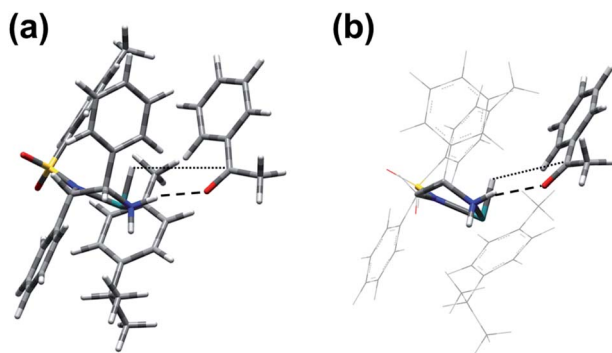
Fig. 8 (a) Pre-organisation of the [Ru( p -cymene)( S,S -TsDPEN-H)]/acetophenone assembly with CO \cdots H _2 N H-bonding (denoted by the dashed line), the initial stage of the catalytic cycle. Note that the vector defined by hydride H and carbonyl C atoms points towards one of the enantiotopic faces of the ketone. (b) Simplified scheme to highlight bonding interactions between catalyst diamine and substrate carbonyl (Fig. S16, PDB13†).
