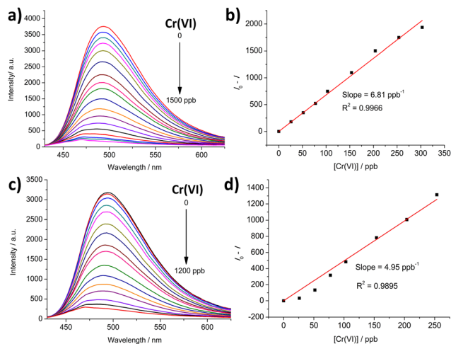
Fig. 11 (a) Fluorescence titration ( \lambda_{\text{exc}} = 400 nm) of acid activated BUT-MOF in suspension ( 0.1 \text{ mg mL}^{-1} ) in distilled water upon the addition of aliquots of a 10^{-4} \text{ M} solution of \text{K}_2\text{Cr}_2\text{O}_7 at pH = 3, (b) calibration curve for the titration in distilled water (black circles correspond to experimental results and the red line corresponds to a linear fit), (c) fluorescence titration ( \lambda_{\text{exc}} = 400 nm) of acid activated BUT-MOF in suspension ( 0.1 \text{ mg mL}^{-1} ) in bottled water upon the addition of aliquots of a 10^{-4} \text{ M} solution of \text{K}_2\text{Cr}_2\text{O}_7 at pH = 3 and (d) calibration curve for the titration in bottled water (black circles correspond to experimental results and the red line corresponds to a linear fit).
