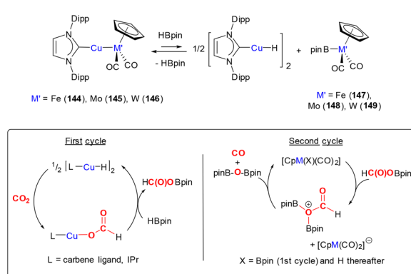
Scheme 43 Mechanism for the 2-electron reduction of CO 2 to CO catalysed by heterobimetallic complexes [(NHC)Cu–ML n ] {ML n = [FeCp(CO) 2 ], [WCp(CO) 3 ], [MoCp(CO) 3 ]}. 168
