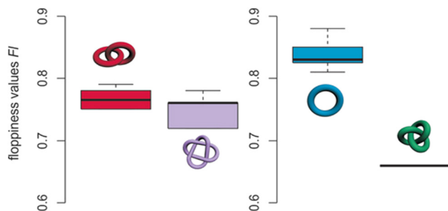
Fig. 29 Floppiness values F for Hopf links (six, left, red), Solomon links (two, left, violet), macrocycles (eight, right, blue), and a trefoil knot (right, green). The box shows the 50% of the range of floppiness values, thick line shows median. Reproduced with permission from Wiley-VCH. 129
