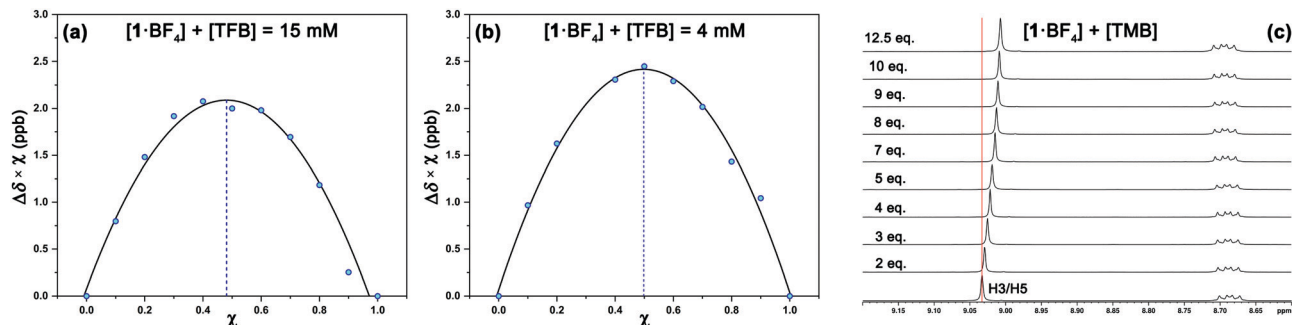
Fig. 6 Representative Job's plots for the interaction of compound 1 and TFB at (a) 15 mM in DMSO- d_6 and (b) 4 mM in acetone- d_6 ; (c) ^1\text{H} NMR titration spectra (500 MHz) of 1 ·BF _4 (20 mM) with TMB in DMSO- d_6 . Key H3/H5 protons are labeled.
