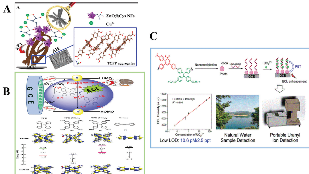
Fig. 6 Schematic illustration of an ECL sensor based on TCPP J-aggregate towards \text{Cu}^{2+} . Adapted from (Han et al. 2020) with permission of Analytical Chemistry , copyright 2020 (A). The mechanism of a designed ECL sensor, molecular orbital amplitude plots and the calculated orbital energy levels for TPE, TPE-(NO 2 ) 4 , TPE-(NH 2 ) 4 and tolane molecules. Adapted from (Han et al. 2019) with permission of Analytical Chemistry , copyright 2019 (B). The assembly of a sensor for uranyl ions. Adapted from (Wang et al. 2020) with permission of Advanced Functional Materials , copyright 2020 (C).
