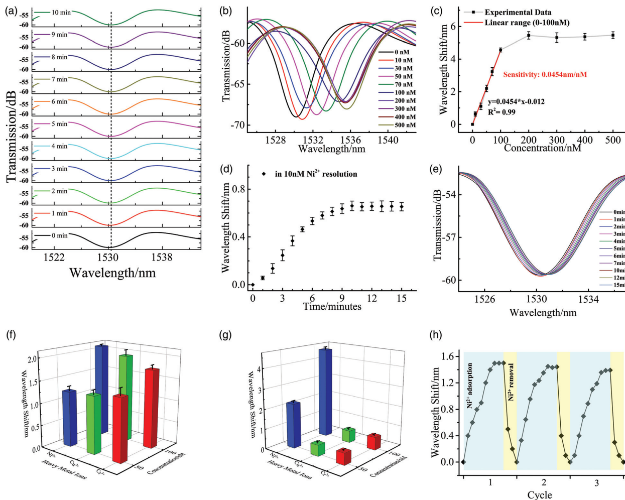
Fig. 3 (a) Spectral response curves of the STNCS sensor coated with Ni 2+ -II-CS and immersed in DI water for 10 min (the standard deviation is 0.098 nm). (b) Spectral response curves of the STNCS sensor coated with Ni 2+ -II-CS to different Ni 2+ ion concentrations. (c) Ni 2+ ion calibration curve and linear response of the STNCS sensor coated with Ni 2+ -II-CS film. (d) Response time curves of the STNCS sensor coated with Ni 2+ -II-CS and immersed in 10 nM Ni 2+ solution. (e) Spectral response of the STNCS sensor coated with Ni 2+ -II-CS to 10 nM Ni 2+ ion solution for 15 min. (f) Response of the STNCS sensor coated with Ni 2+ -NII-CS to different concentrations (50 and 100 nM) of heavy metal ions (nickel, copper, and chromium). (g) Response of the STNCS sensor coated with Ni 2+ -II-CS to different concentrations (50 and 100 nM) of heavy metal ions (nickel, copper, and chromium). (Error bars represent standard deviations for three parallel experiments). (h) Regeneration cycle: shift in dip wavelength of the STNCS sensor coated with Ni 2+ -II-CS caused by sequential exposure to 50 nM Ni 2+ solution and MES buffer.
