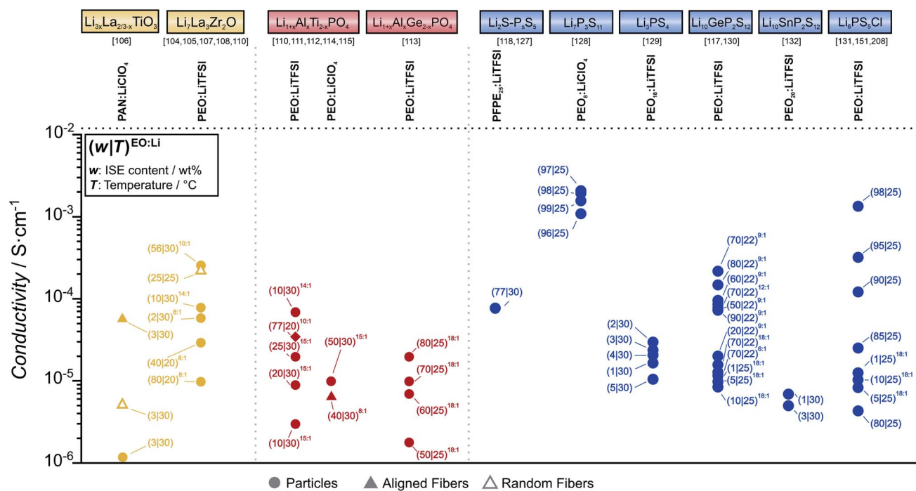
Fig. 8 Ionic conductivity survey of oxide- (yellow), phosphate- (red) and thiophosphate-based (blue) particle-in-polymer or fiber-in-polymer composite electrolytes. Data for different polymers, conducting salt and ISE morphology/microstructure are shown. Measurement temperature and composition of the composite electrolyte are highlighted for each point.
