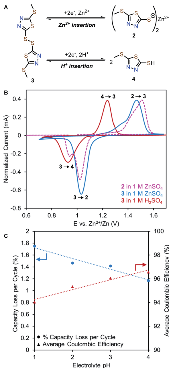
Fig. 5 (A) Possible \text{Zn}^{2+} and \text{H}^+ insertion products derived from reduction of 3 . (B) Solid state CV of 2 measured in a two-electrode cell with 1 M \text{ZnSO}_4 electrolyte (pink dotted line) and 3 measured in a three-electrode cell with 1 M \text{ZnSO}_4 (blue solid line) or 1 M \text{H}_2\text{SO}_4 electrolytes (red solid line). The position of the 1 M \text{H}_2\text{SO}_4 curve is adjusted to represent a dilute \text{H}_2\text{SO}_4 solution (pH = 4), calculated based on the Nernst equation. Current is normalized to oxidation peak for consistency. (C) pH-dependent capacity loss and coulombic efficiency of Zn-2 cells.
